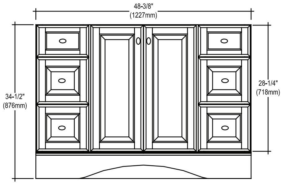
3. Front view line drawing
