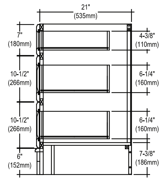
4. Side view line drawing
